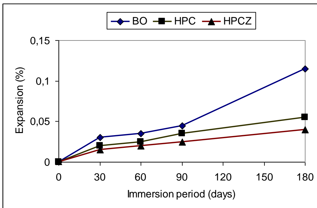
Fig 7: Expansion of the concrete specimens immersed in the solution containing 5% \text{NH}_4\text{SO}_4 ammonium sulphate
