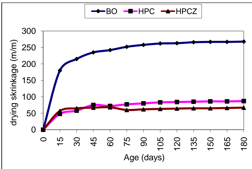
Fig 8: Autogenous skrinkage of different kinds of concrete.
