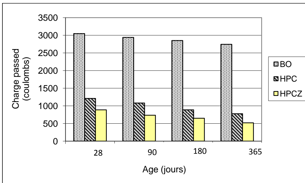
Fig 6: Charge passed in the concrete specimen kept in the sulphated environment
